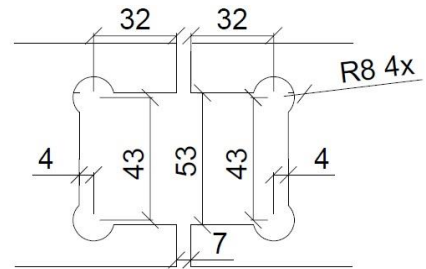
Glas Cut-Out
