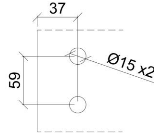
Glas Cut-Out
