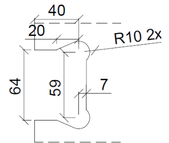
Glas Cut-Out
