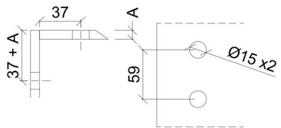
Glas Cut-Out
