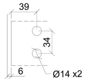
Glas Cut-Out
