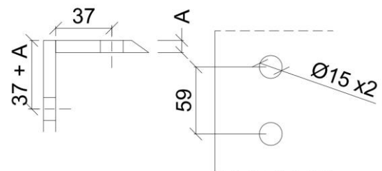
Glas Cut-Out
