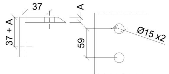
Glas Cut-Out
