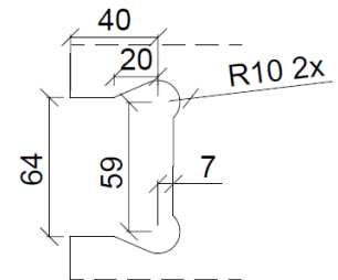
Glas Cut-Out
