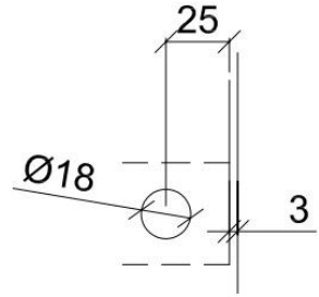
Glas Cut-Out
