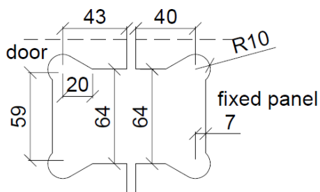
Glas Cut-Out
