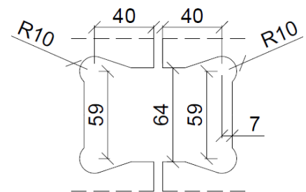
Glas Cut-Out
