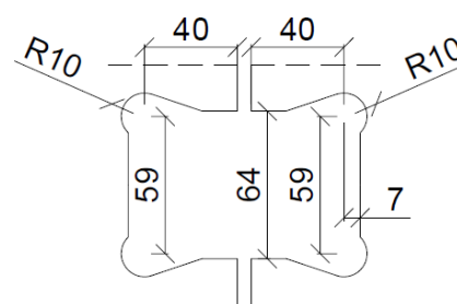
Glas Cut-Out
