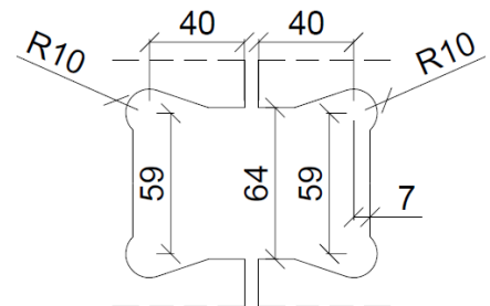
Glas Cut-Out
