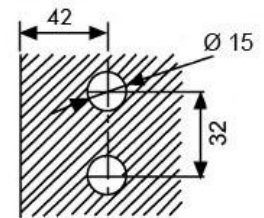
Glas Cut-Out
