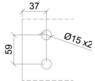
Glas Cut-Out
