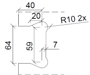
Glas Cut-Out
