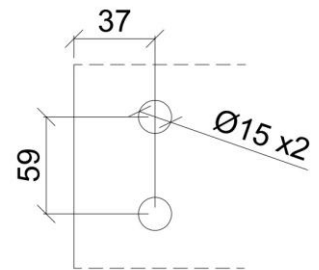
Glas Cut-Out
