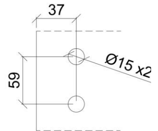
Glas Cut-Out
