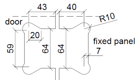
Glas Cut-Out
