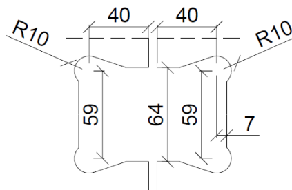
Glas Cut-Out
