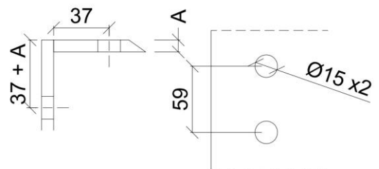
Glas Cut-Out
