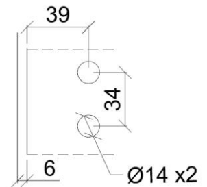
Glas Cut-Out
