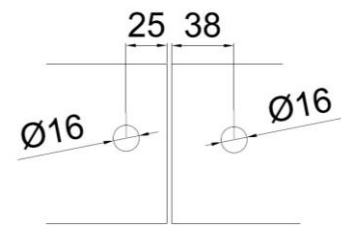
Glas Cut-Out
