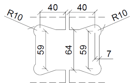
Glas Cut-Out
