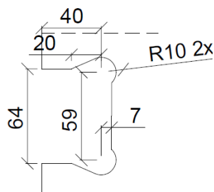
Glas Cut-Out
