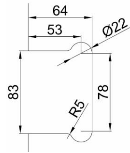
Glas Cut-Out
