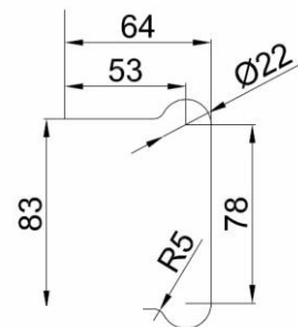
Glas Cut-Out
