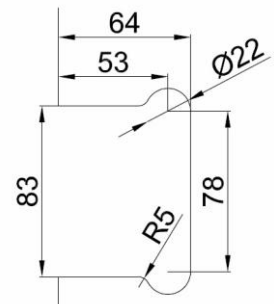
Glas Cut-Out
