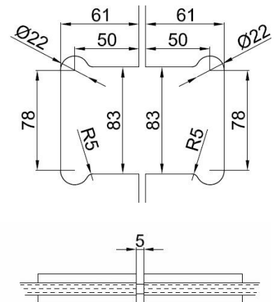
Glas Cut-Out
